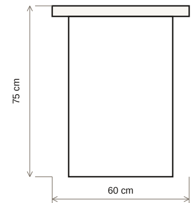
SIDE ELEVATION
